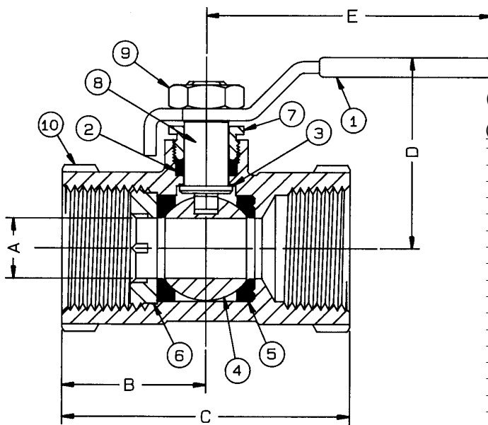
CARBON STEEL UNI-BODY SATURN® BALL VALVE
