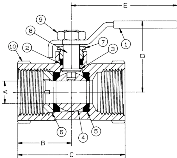
BRONZE UNI-BODY SATURN® BALL VALVE
