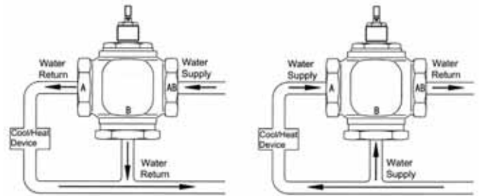
Diverting 3-way
